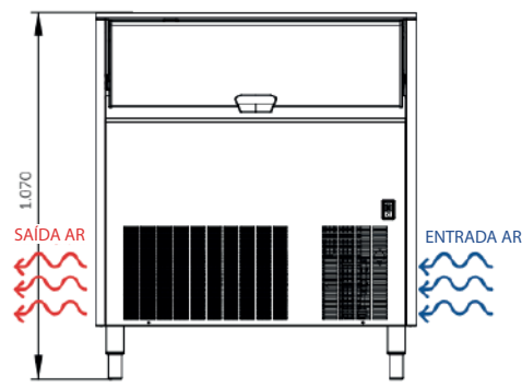
VISTA FRONTAL
