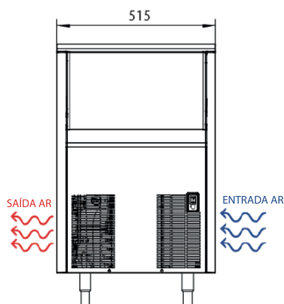
VISTA FRONTAL
